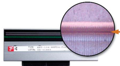
After cleaning 60X magnification reveals a clean burnline free of debris
