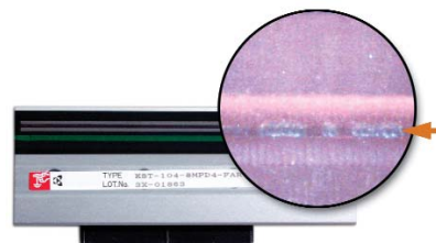
60X magnification shows heavy build-up of debris along the printhead burnline.
